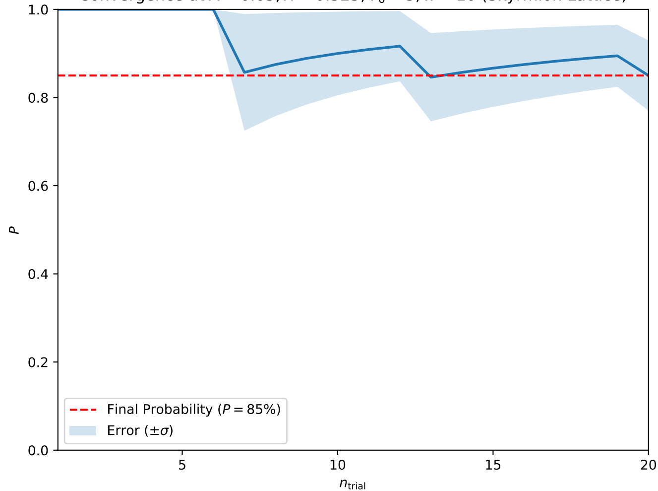
Convergence at A = 0.05, H = 0.325, T_0 = 3, w = 10 (Skyrmion Lattice)
