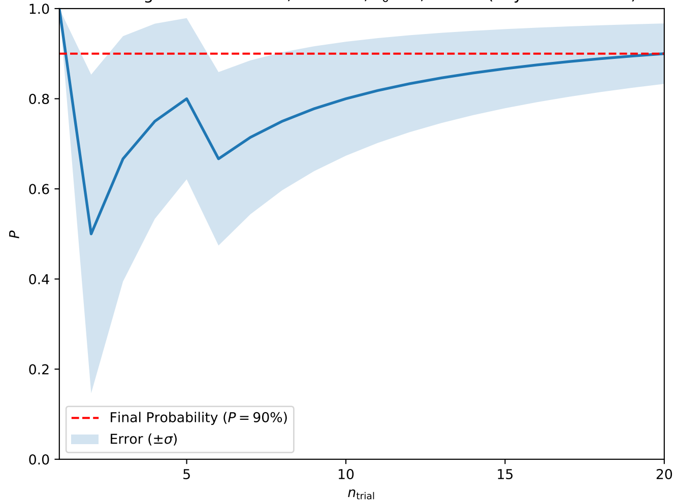
Convergence at A = 0.05, H = 0.35, T_0 = 3, w = 10 (Skyrmion Lattice)
