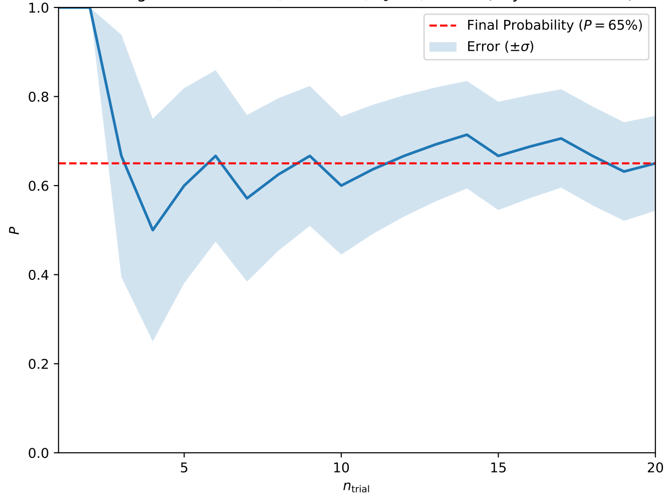
Convergence at A = 0.05, H = 0.375, T_0 = 3, w = 10 (Skyrmion Lattice)
