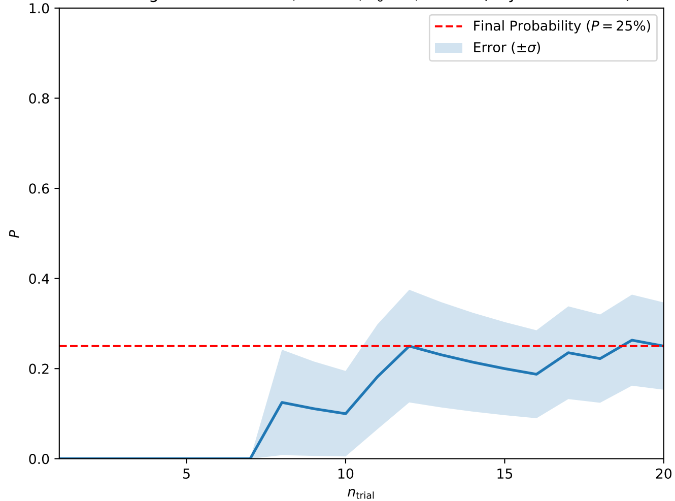
Convergence at A = 0.05, H = 0.4, T_0 = 3, w = 10 (Skyrmion Lattice)
