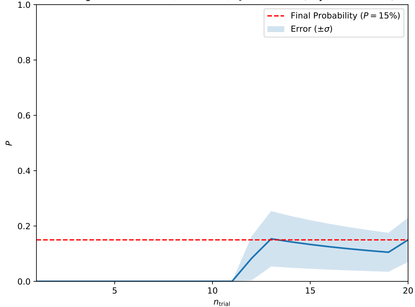
Convergence at A = 0.05, H = 0.425, T_0 = 3, w = 10 (Skyrmion Lattice)
