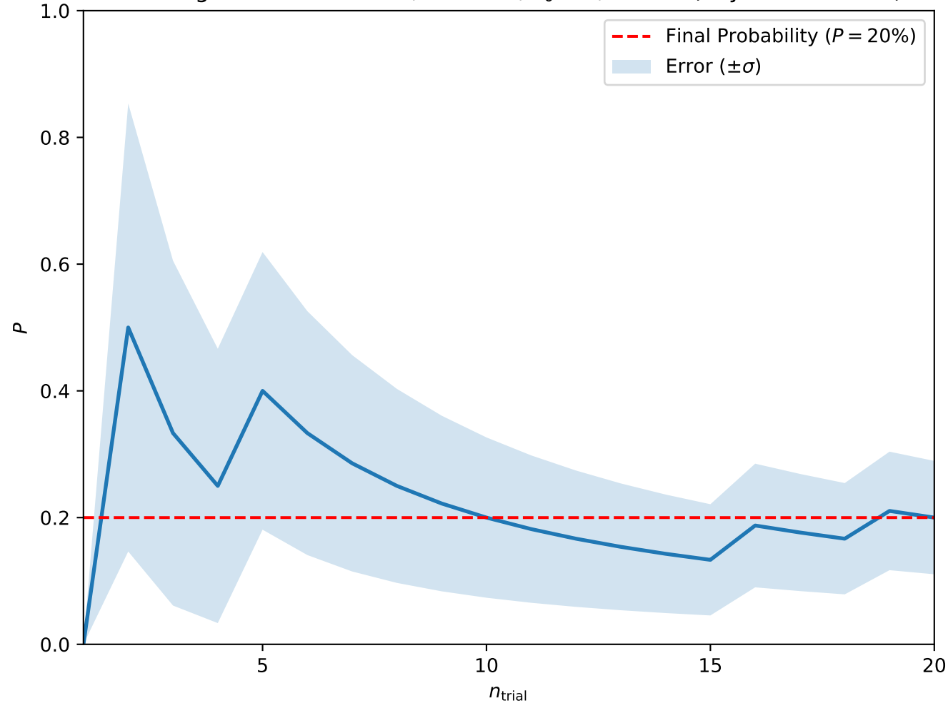
Convergence at A = 0.075, H = 0.25, T_0 = 3, w = 10 (Skyrmion Lattice)
