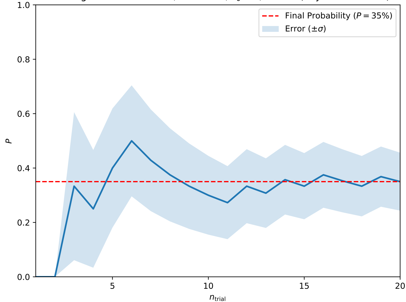
Convergence at A = 0.075, H = 0.275, T_0 = 3, w = 10 (Skyrmion Lattice)
