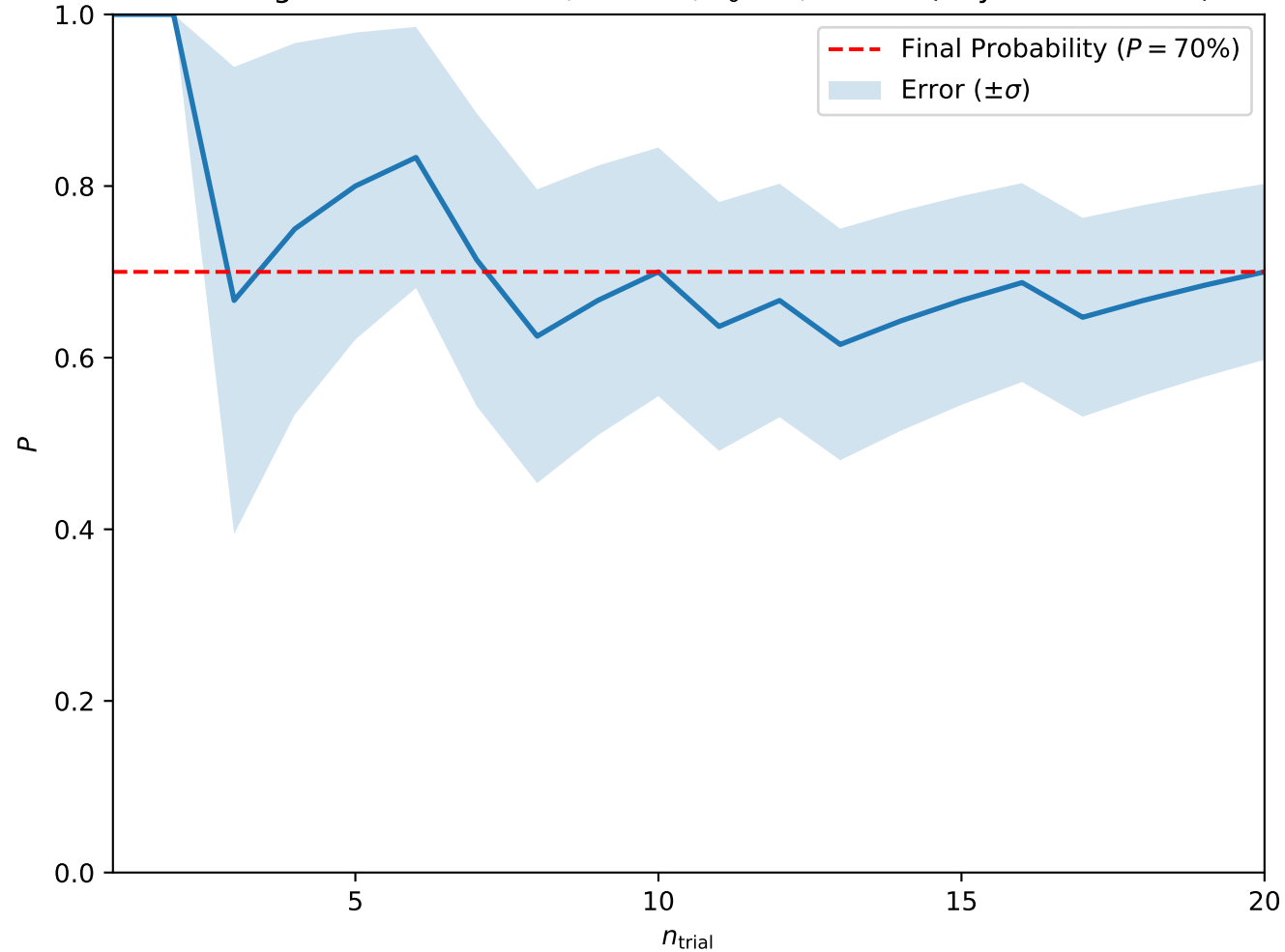
Convergence at A = 0.075, H = 0.3, T_0 = 3, w = 10 (Skyrmion Lattice)
