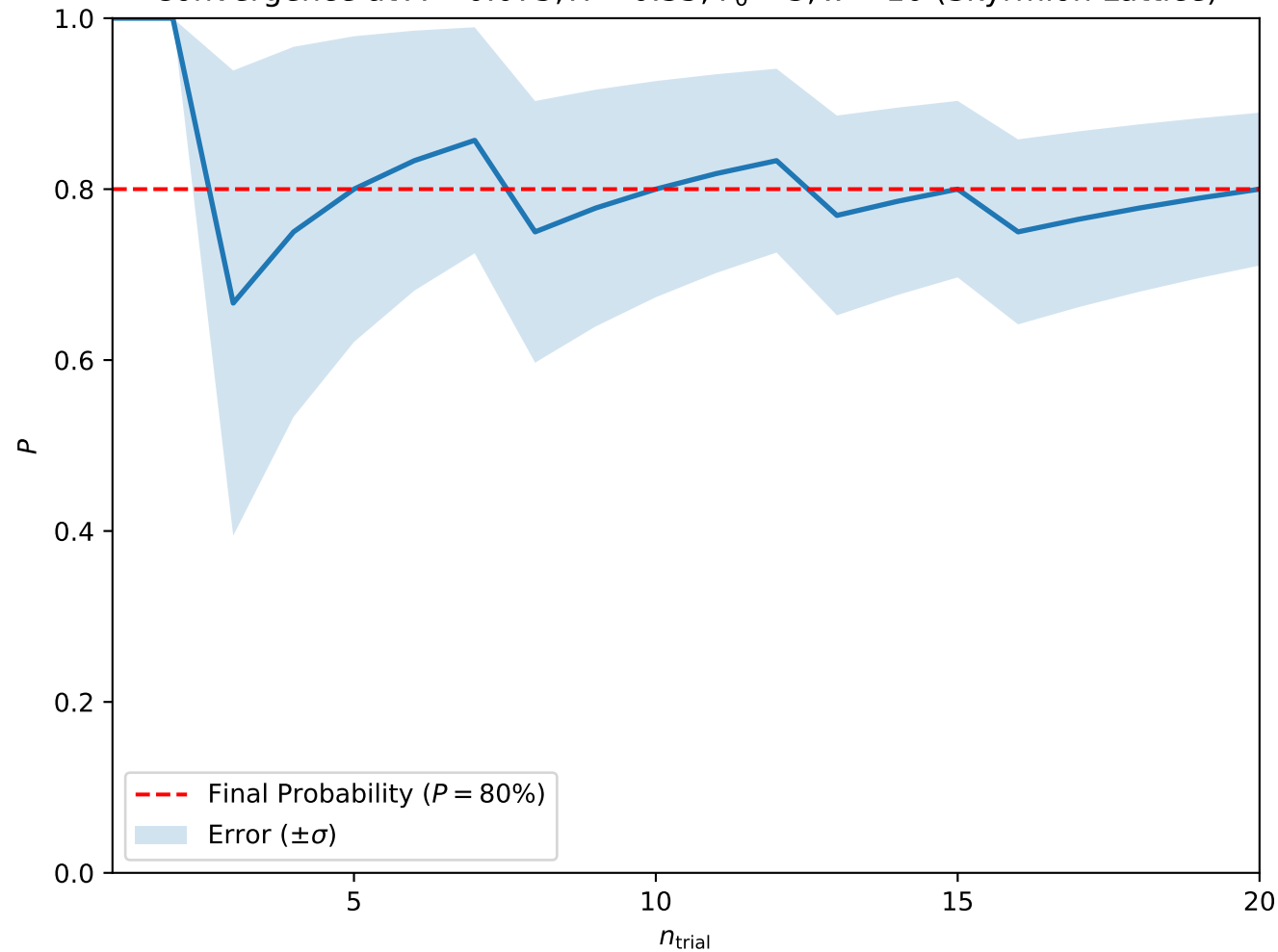
Convergence at A = 0.075, H = 0.35, T_0 = 3, w = 10 (Skyrmion Lattice)
