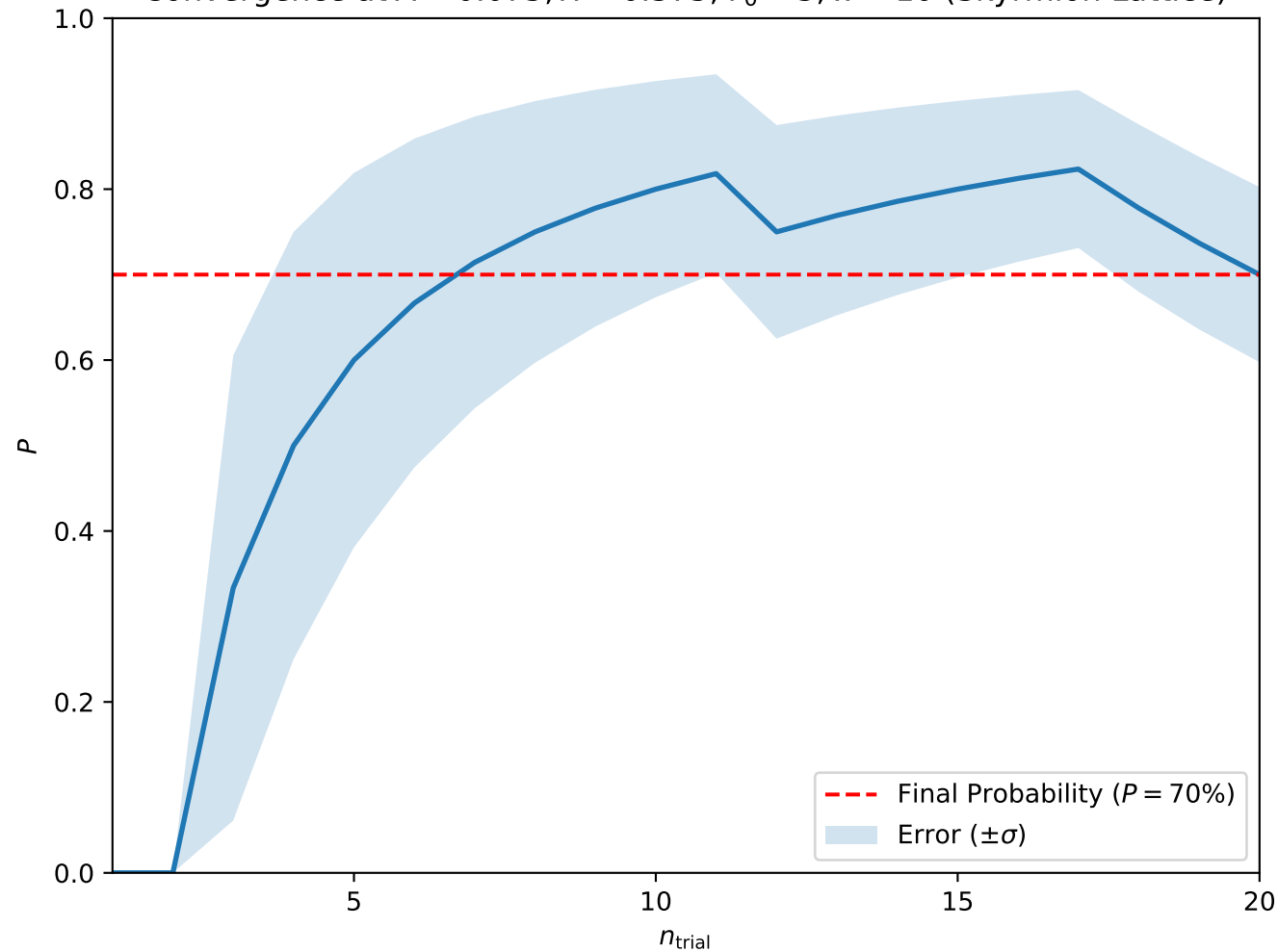
Convergence at A = 0.075, H = 0.375, T_0 = 3, w = 10 (Skyrmion Lattice)
