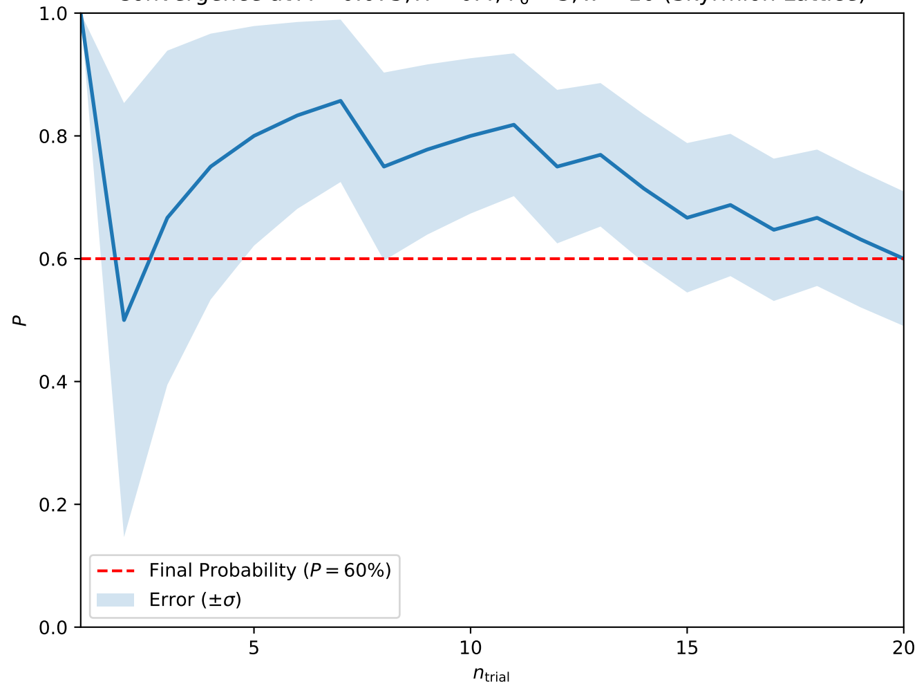
Convergence at A = 0.075, H = 0.4, T_0 = 3, w = 10 (Skyrmion Lattice)
