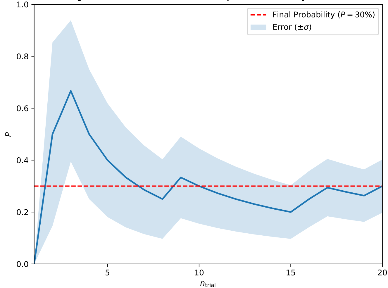
Convergence at A = 0.075, H = 0.425, T_0 = 3, w = 10 (Skyrmion Lattice)
