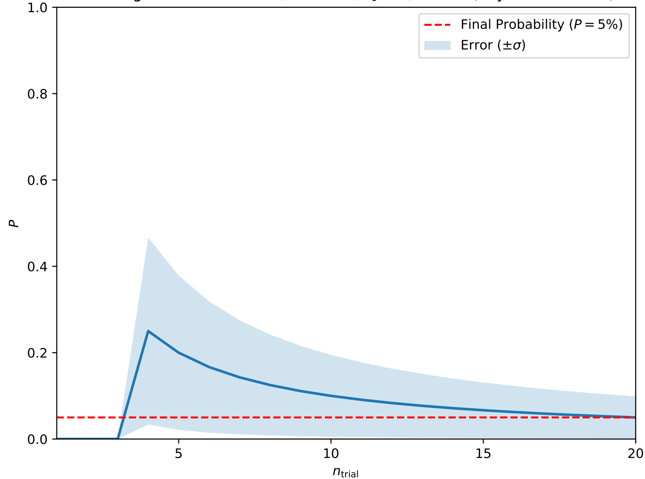
Convergence at A = 0.075, H = 0.45, T_0 = 3, w = 10 (Skyrmion Lattice)
