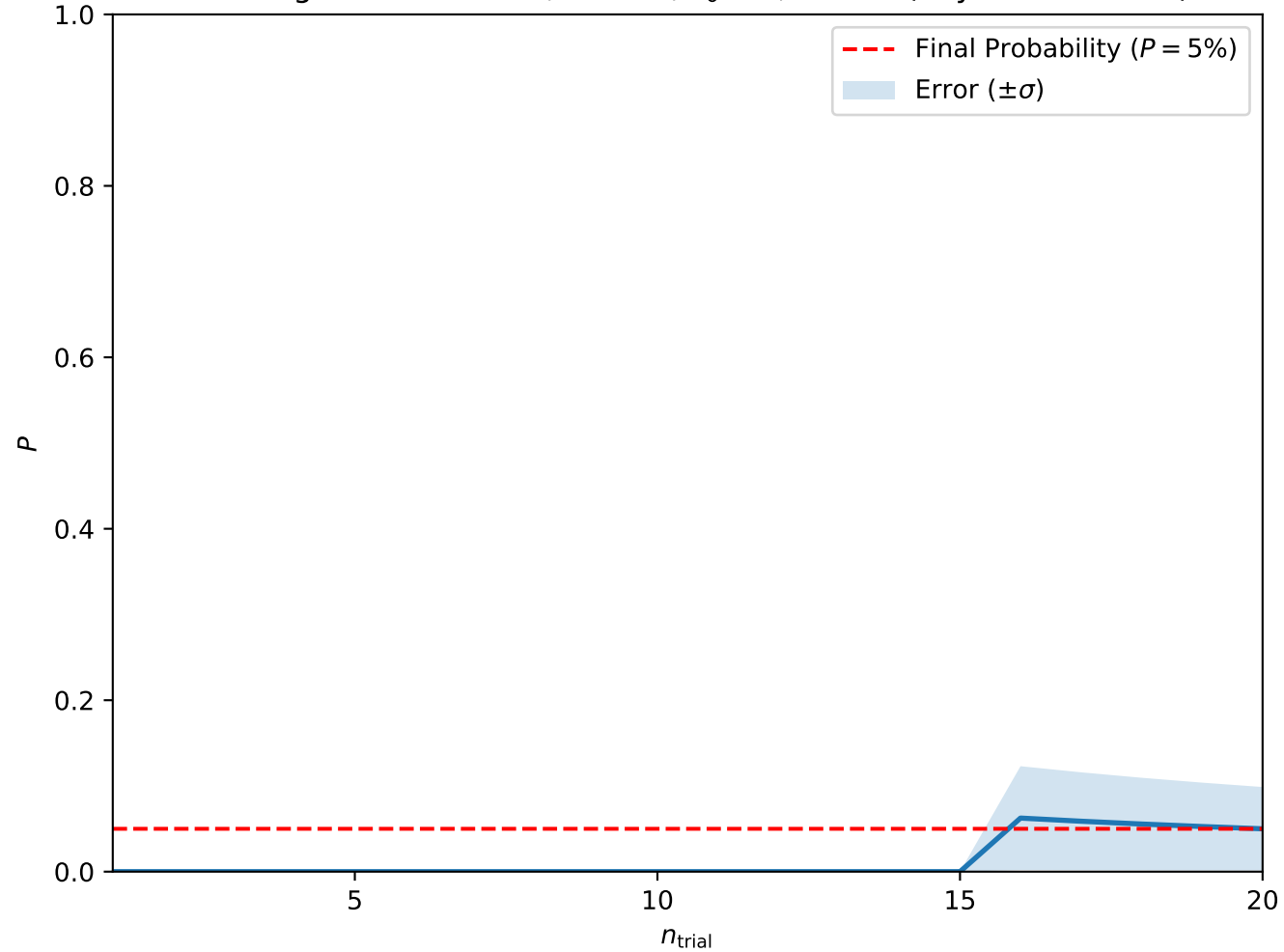
Convergence at A = 0.0, H = 0.2, T_0 = 3, w = 10 (Skyrmion Lattice)
