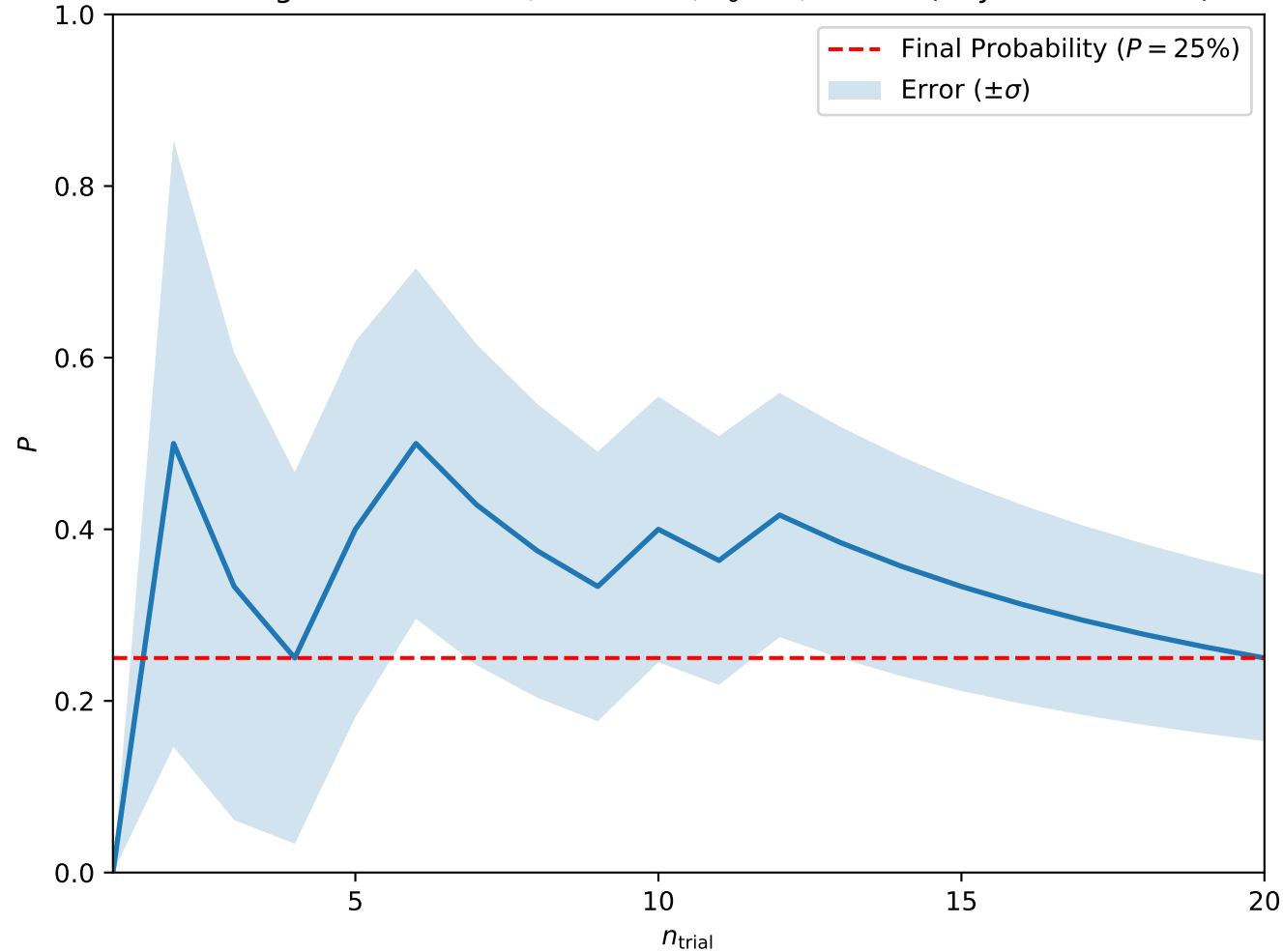
Convergence at A = 0.0, H = 0.225, T_0 = 3, w = 10 (Skyrmion Lattice)
