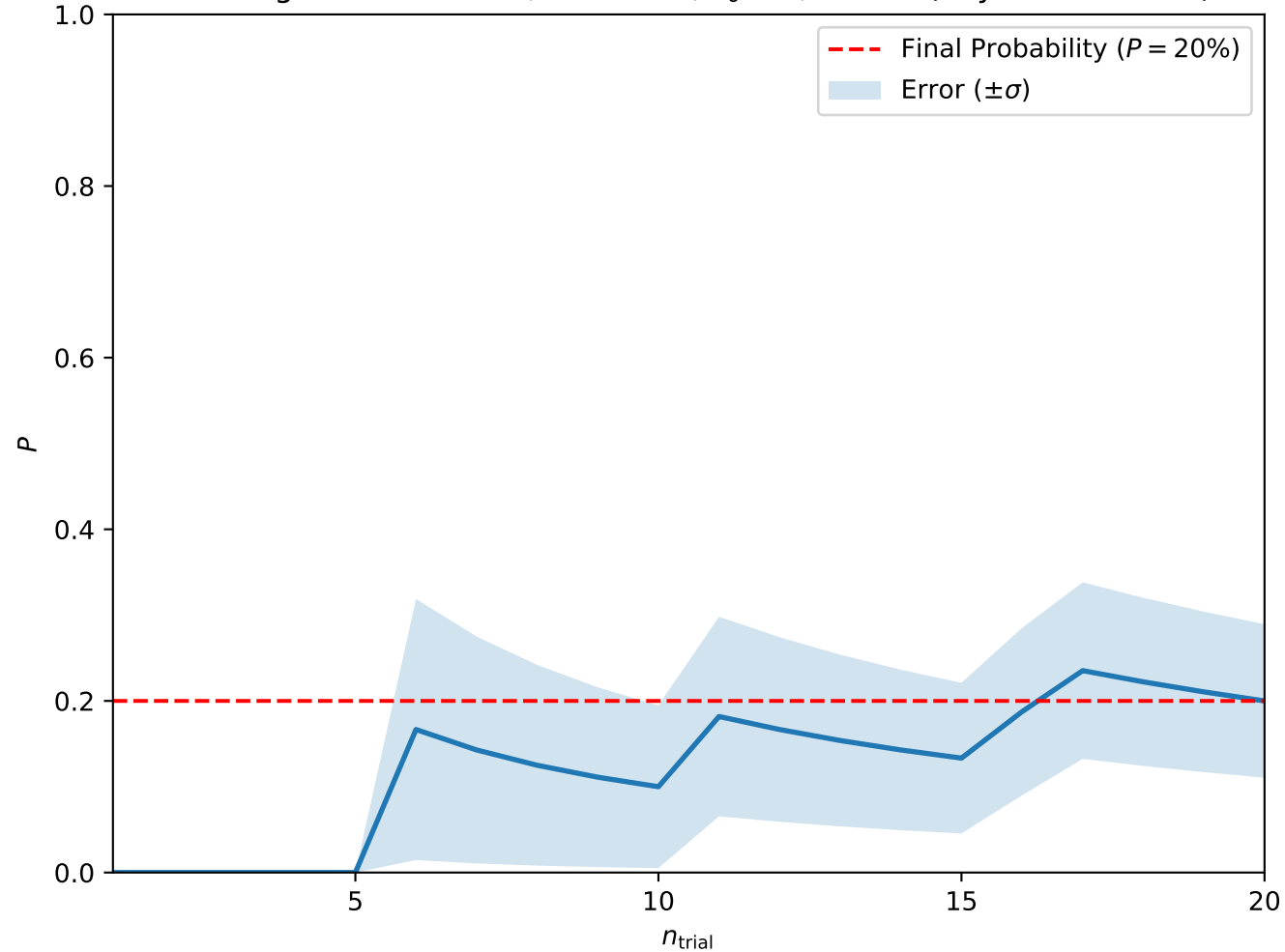
Convergence at A = 0.0, H = 0.275, T_0 = 3, w = 10 (Skyrmion Lattice)
