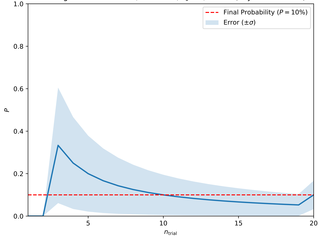
Convergence at A = 0.125, H = 0.225, T_0 = 3, w = 10 (Skyrmion Lattice)
