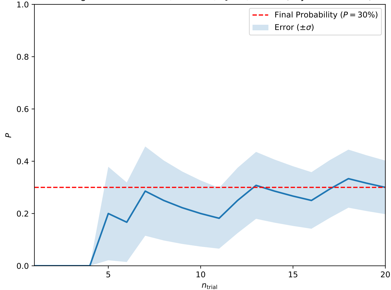
Convergence at A = 0.125, H = 0.25, T_0 = 3, w = 10 (Skyrmion Lattice)
