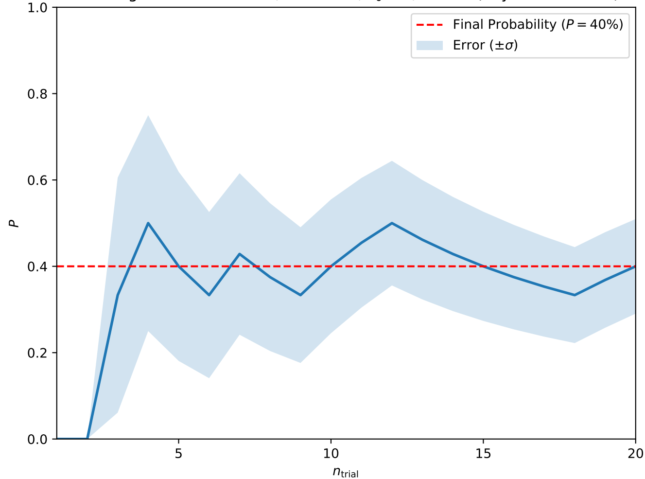
Convergence at A = 0.125, H = 0.275, T_0 = 3, w = 10 (Skyrmion Lattice)
