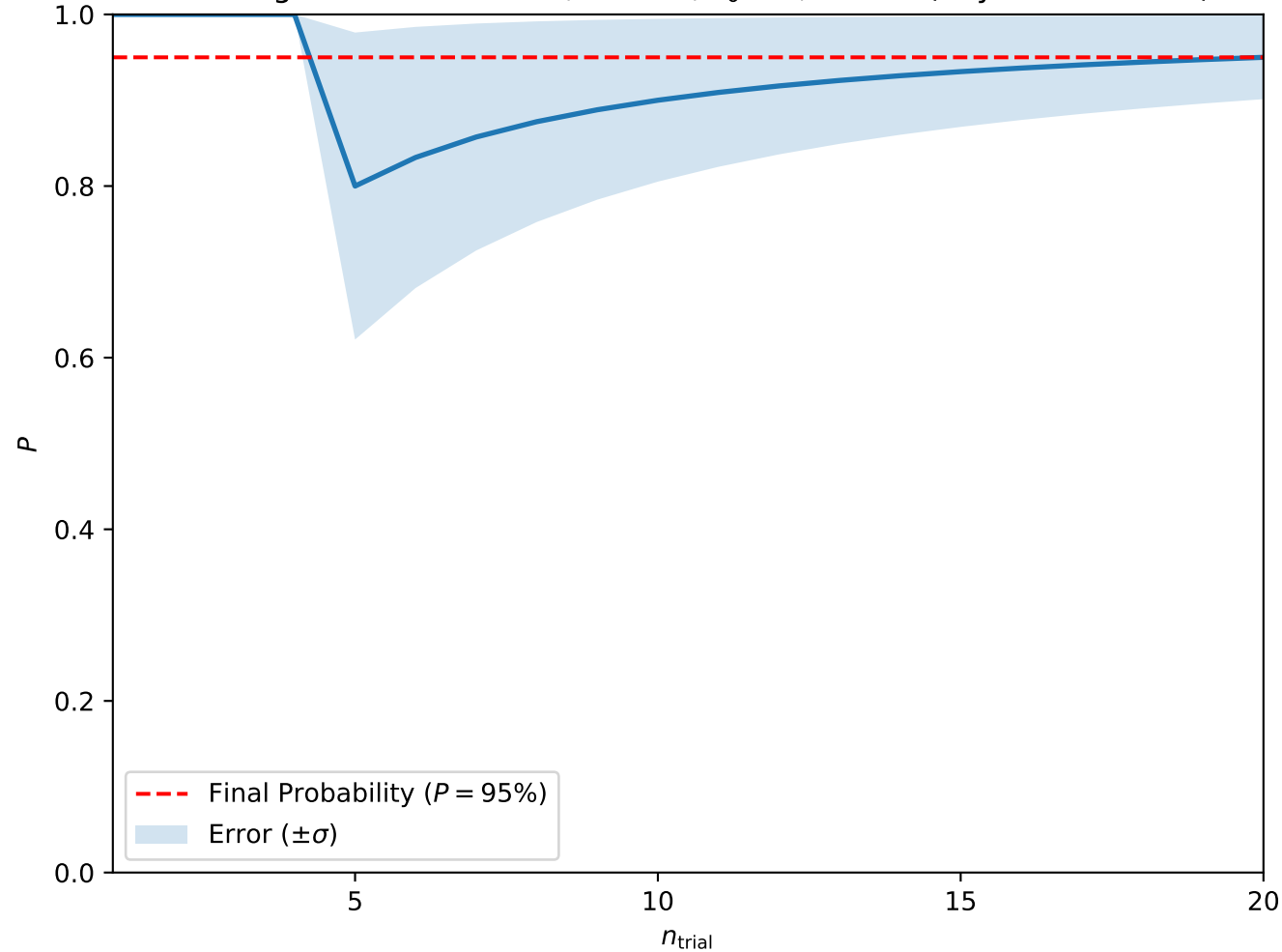
Convergence at A = 0.125, H = 0.3, T_0 = 3, w = 10 (Skyrmion Lattice)
