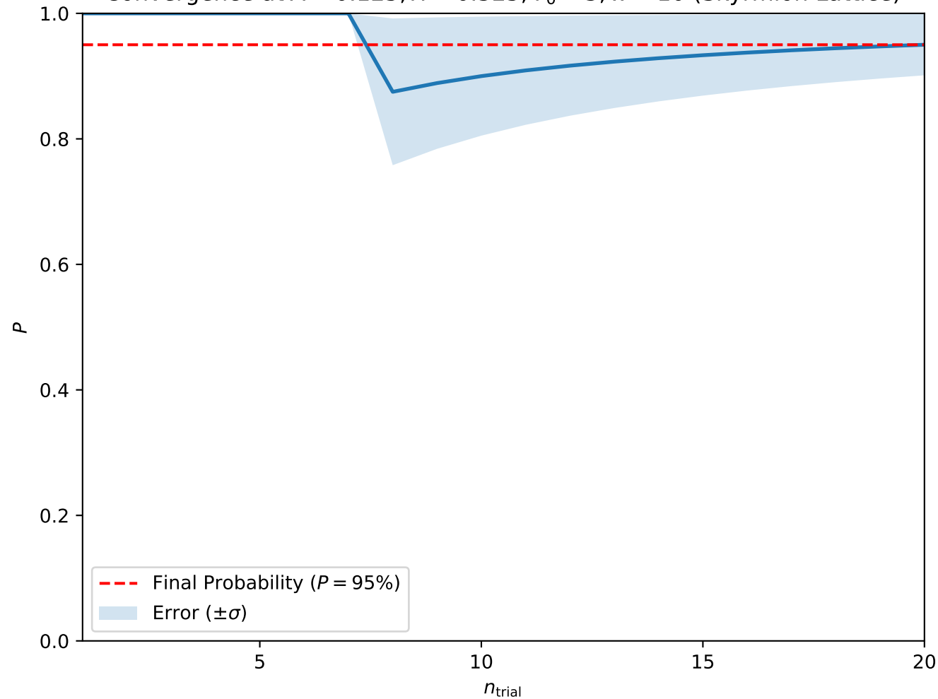
Convergence at A = 0.125, H = 0.325, T_0 = 3, w = 10 (Skyrmion Lattice)
