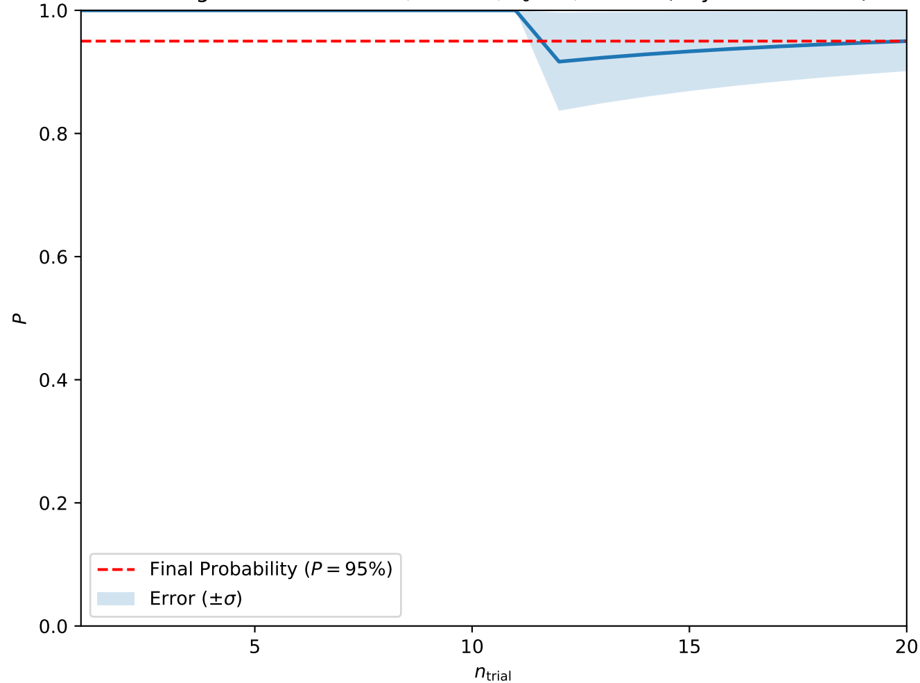
Convergence at A = 0.125, H = 0.4, T_0 = 3, w = 10 (Skyrmion Lattice)
