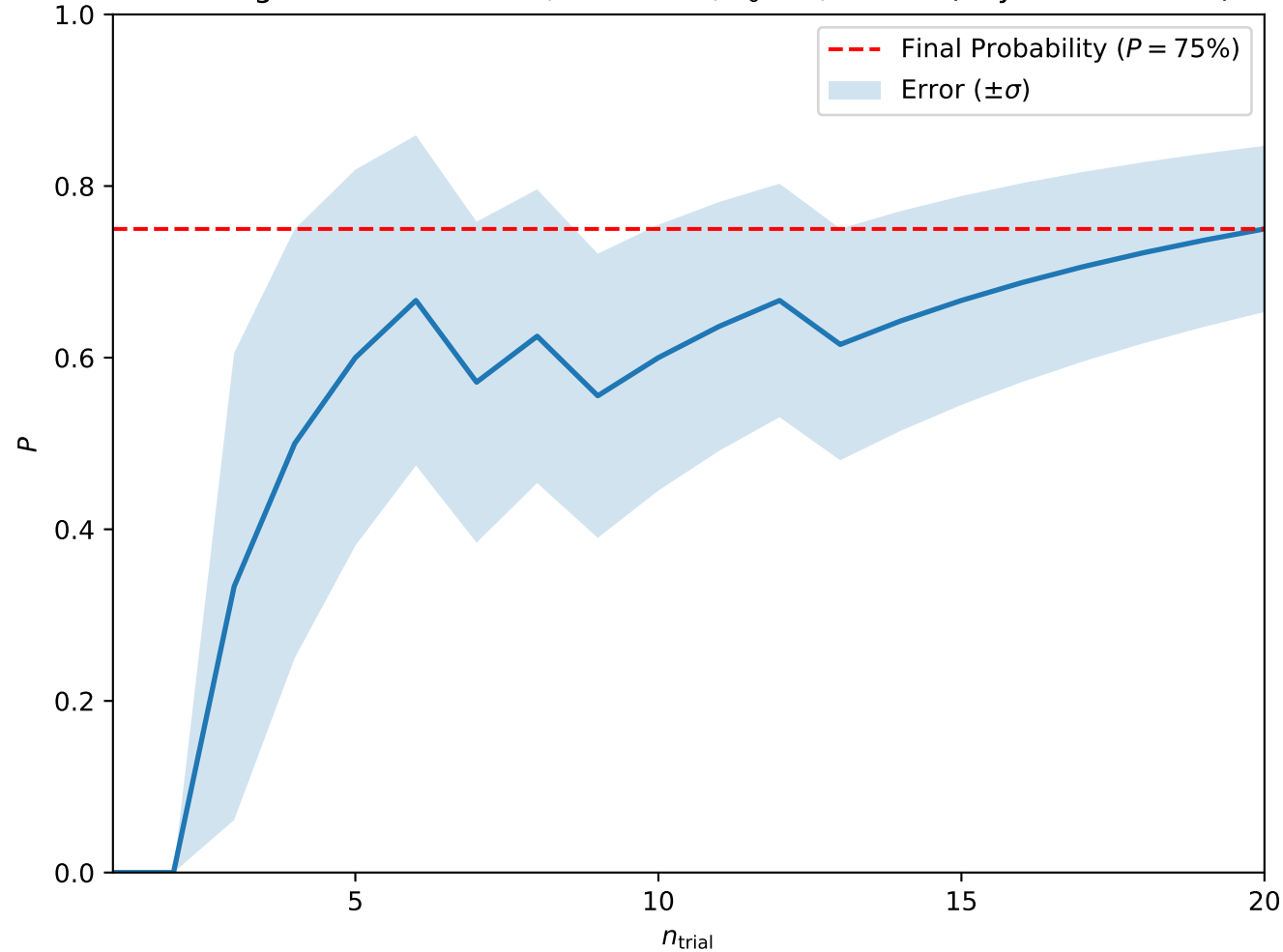
Convergence at A = 0.125, H = 0.425, T_0 = 3, w = 10 (Skyrmion Lattice)
