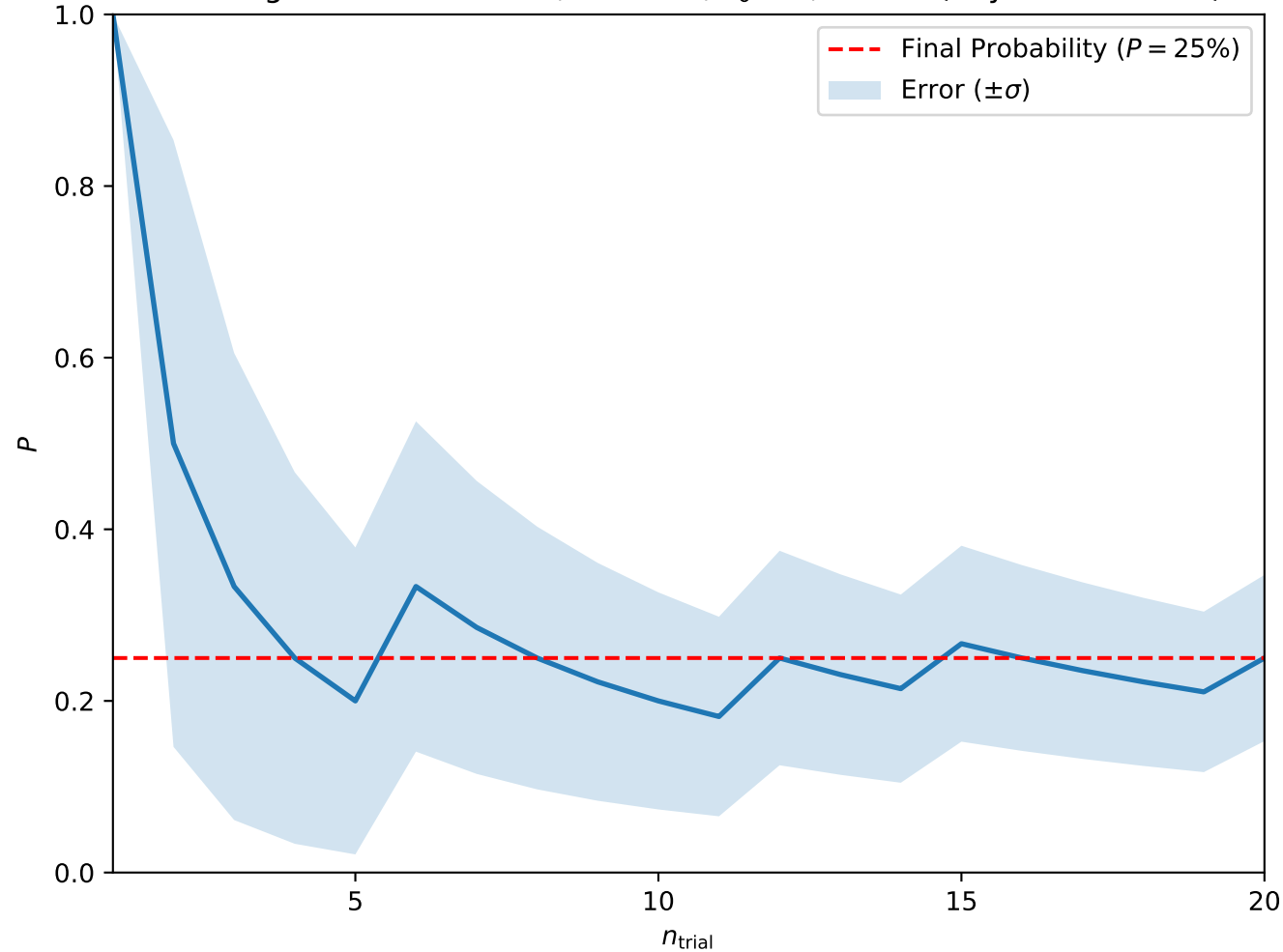
Convergence at A = 0.125, H = 0.45, T_0 = 3, w = 10 (Skyrmion Lattice)
