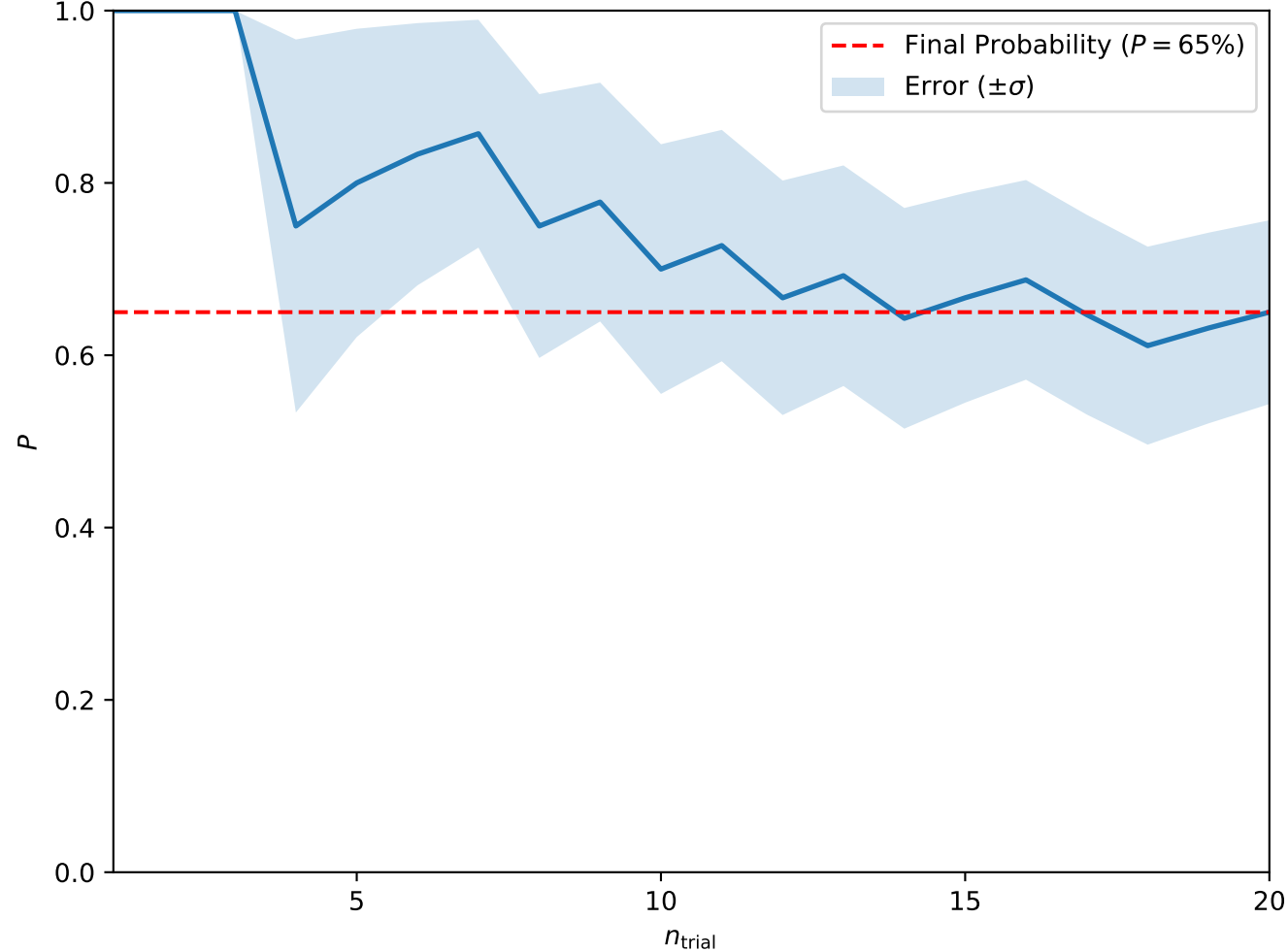
Convergence at A = 0.15, H = 0.3, T_0 = 3, w = 10 (Skyrmion Lattice)
