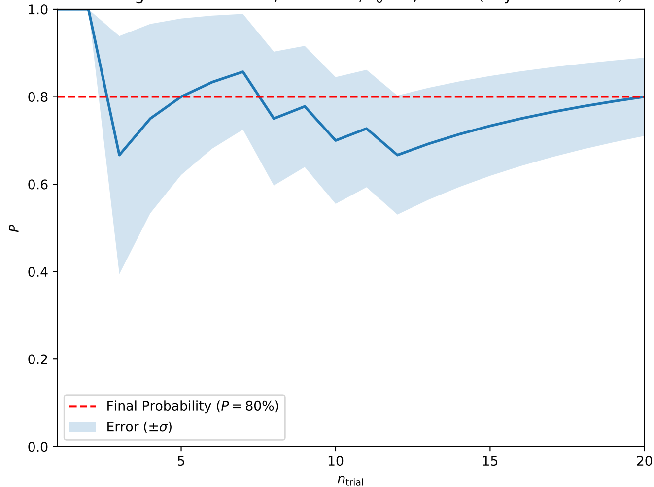
Convergence at A = 0.15, H = 0.425, T_0 = 3, w = 10 (Skyrmion Lattice)
