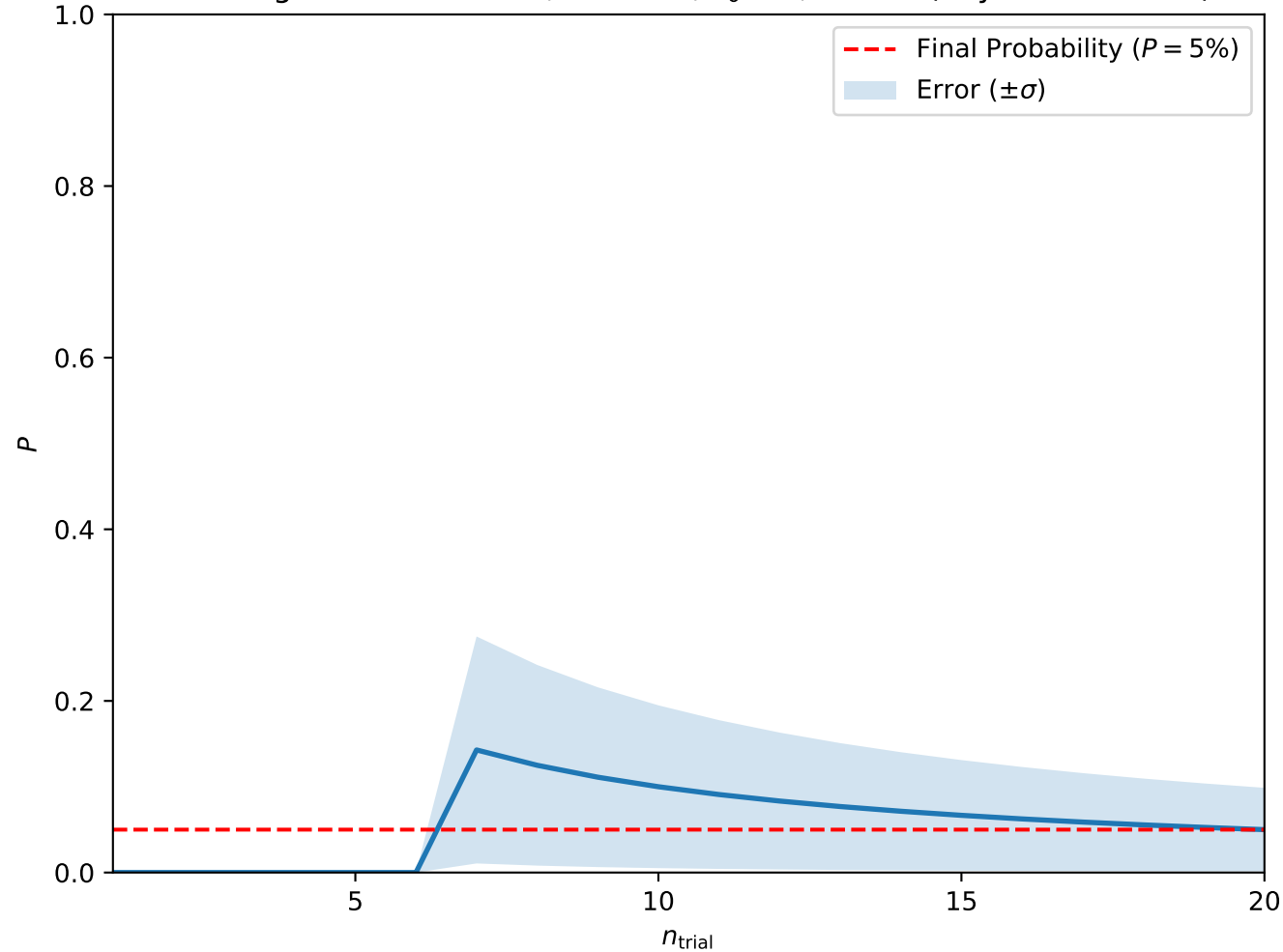
Convergence at A = 0.15, H = 0.45, T_0 = 3, w = 10 (Skyrmion Lattice)
