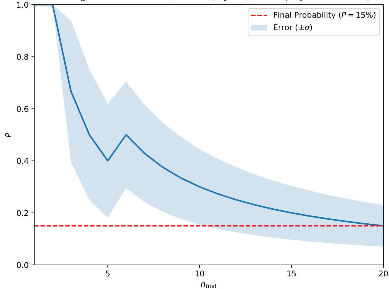
Convergence at A = 0.175, H = 0.25, T_0 = 3, w = 10 (Skyrmion Lattice)
