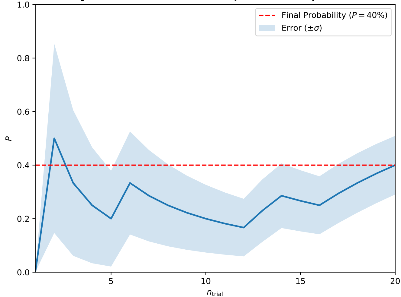
Convergence at A = 0.175, H = 0.275, T_0 = 3, w = 10 (Skyrmion Lattice)
