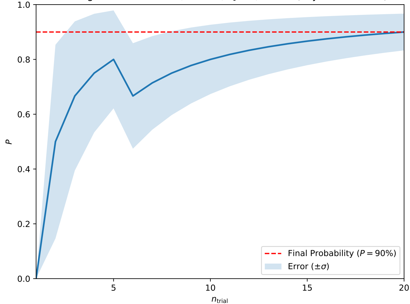
Convergence at A = 0.175, H = 0.4, T_0 = 3, w = 10 (Skyrmion Lattice)
