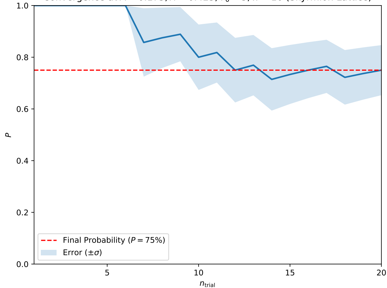
Convergence at A = 0.175, H = 0.425, T_0 = 3, w = 10 (Skyrmion Lattice)
