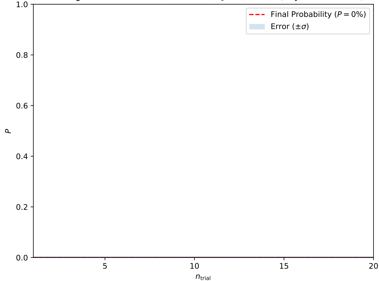
Convergence at A = 0.175, H = 0.575, T_0 = 3, w = 10 (Skyrmion Lattice)
