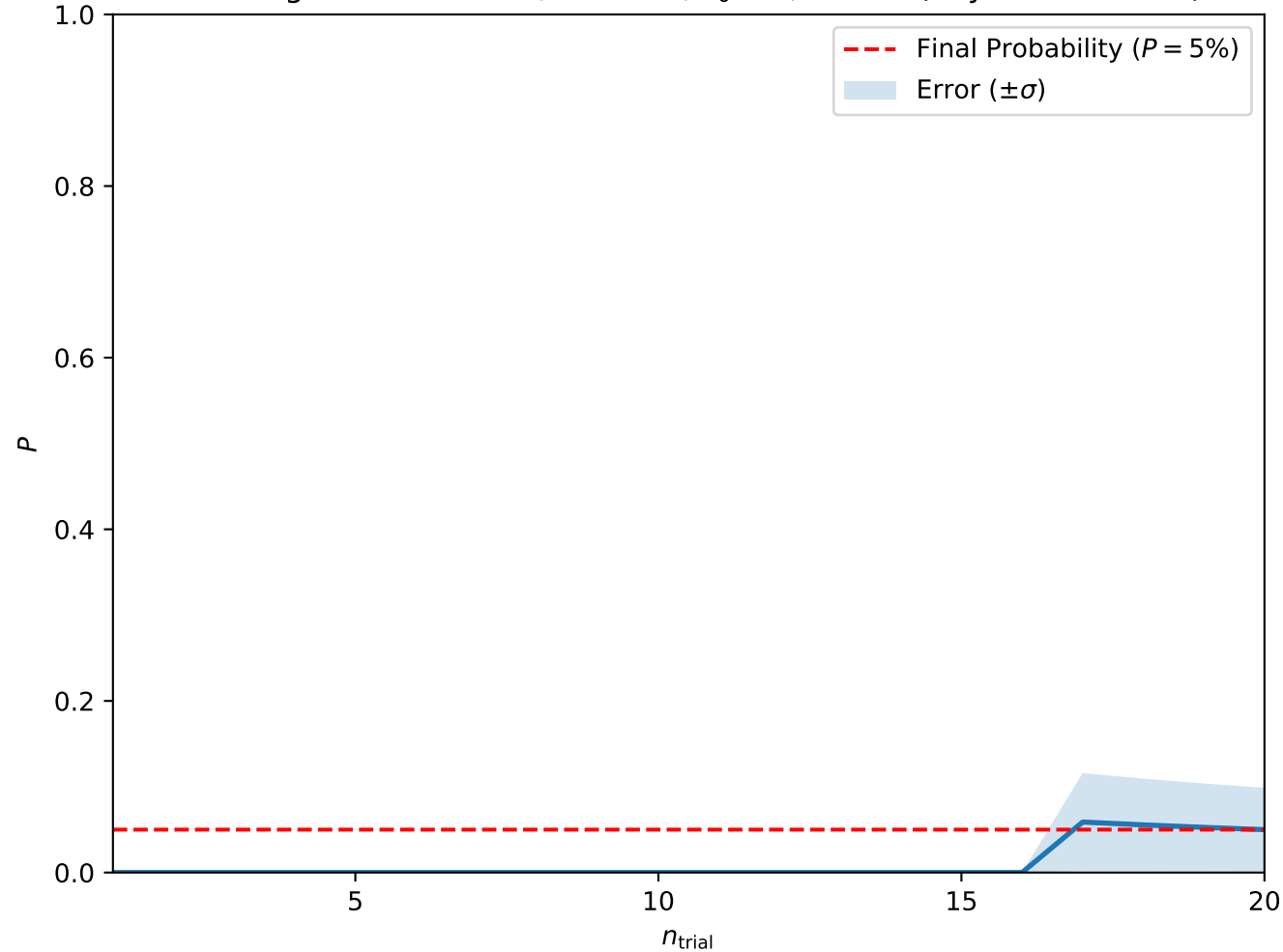
Convergence at A = 0.1, H = 0.25, T_0 = 3, w = 10 (Skyrmion Lattice)
