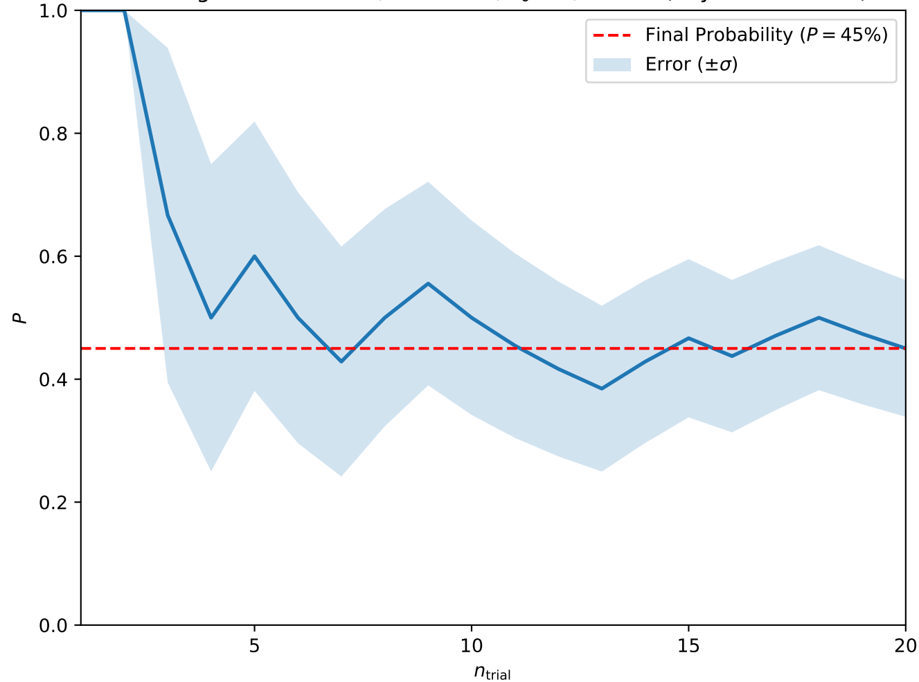
Convergence at A = 0.1, H = 0.275, T_0 = 3, w = 10 (Skyrmion Lattice)
