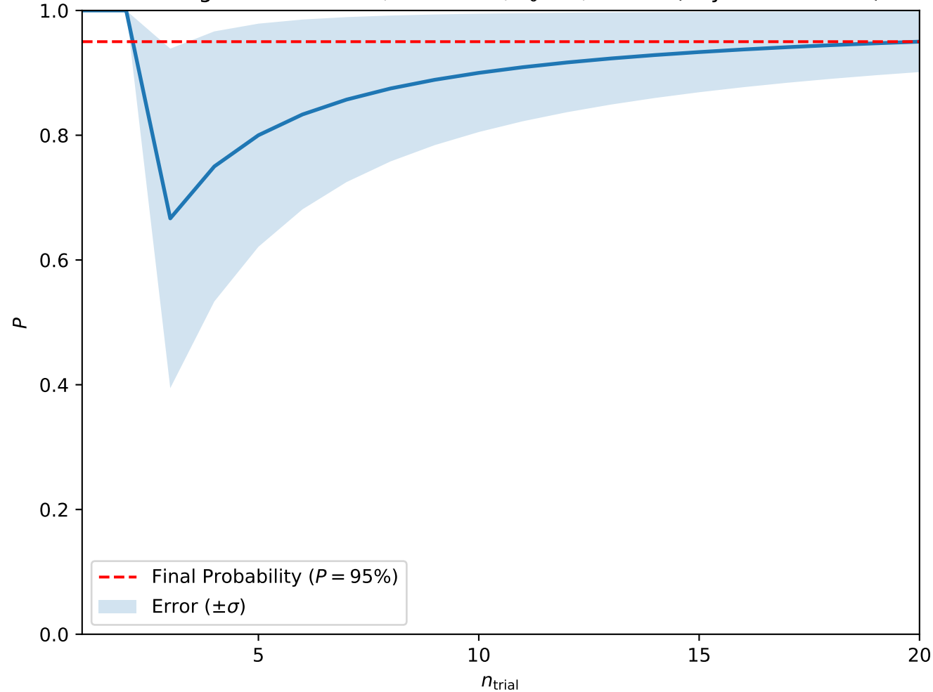
Convergence at A = 0.1, H = 0.325, T_0 = 3, w = 10 (Skyrmion Lattice)
