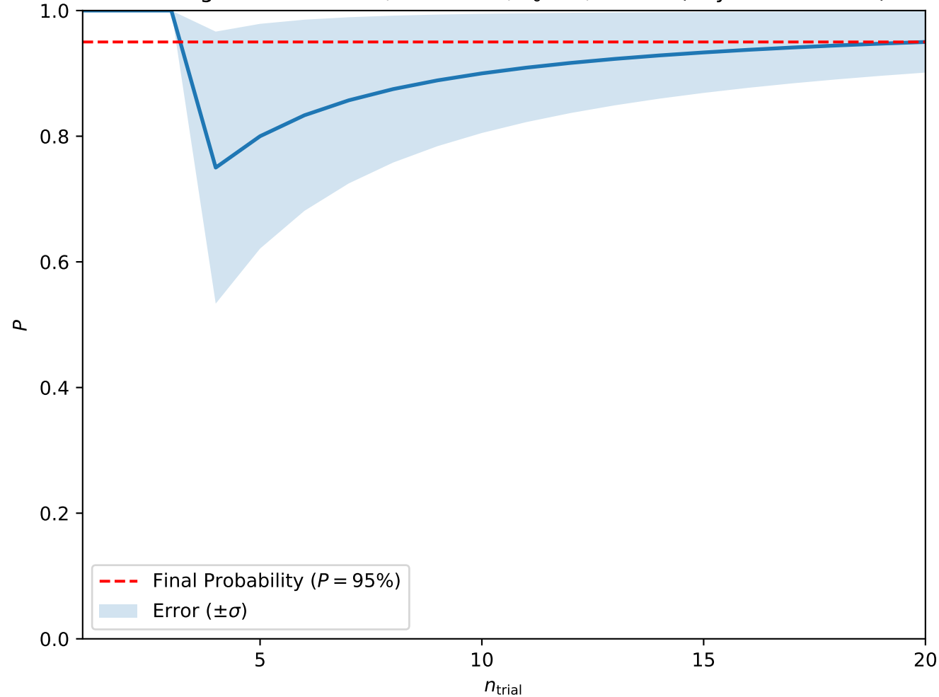
Convergence at A = 0.1, H = 0.375, T_0 = 3, w = 10 (Skyrmion Lattice)
