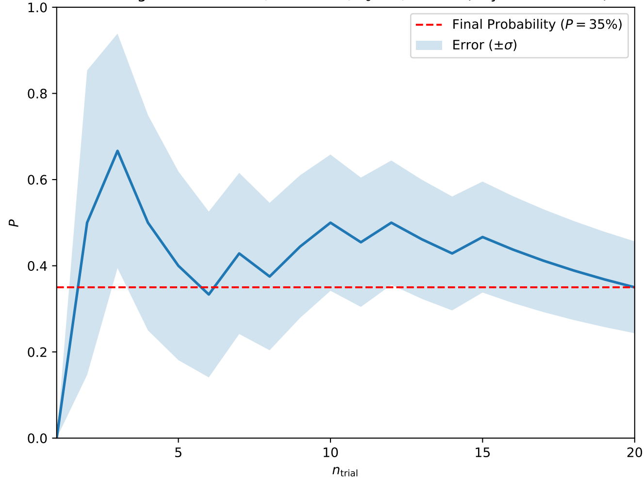
Convergence at A = 0.1, H = 0.425, T_0 = 3, w = 10 (Skyrmion Lattice)
