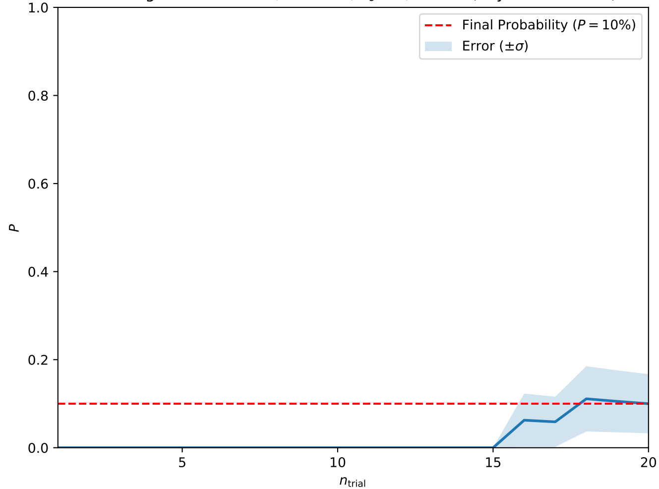
Convergence at A = 0.1, H = 0.45, T_0 = 3, w = 10 (Skyrmion Lattice)
