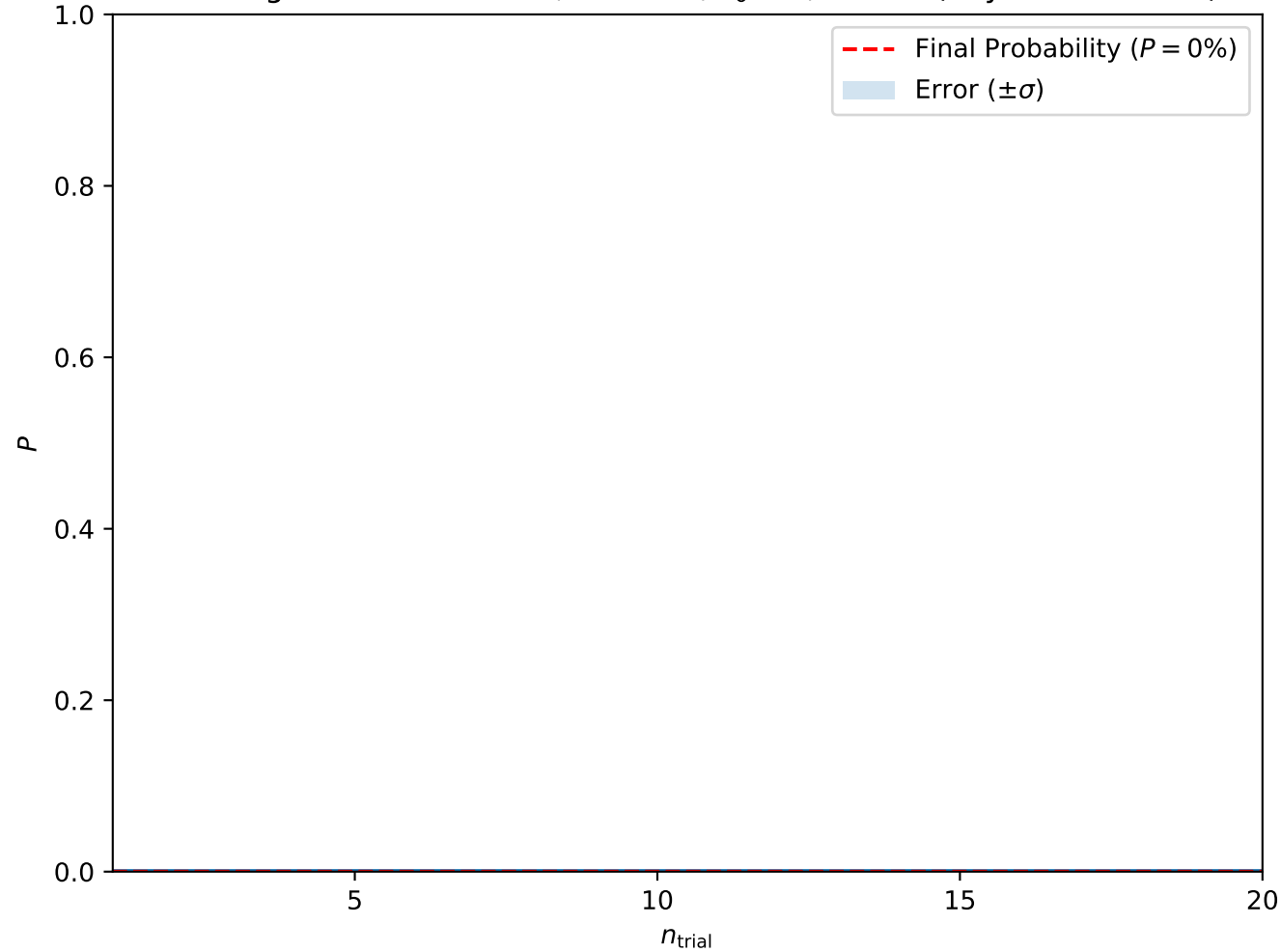
Convergence at A = 0.225, H = 0.25, T_0 = 3, w = 10 (Skyrmion Lattice)
