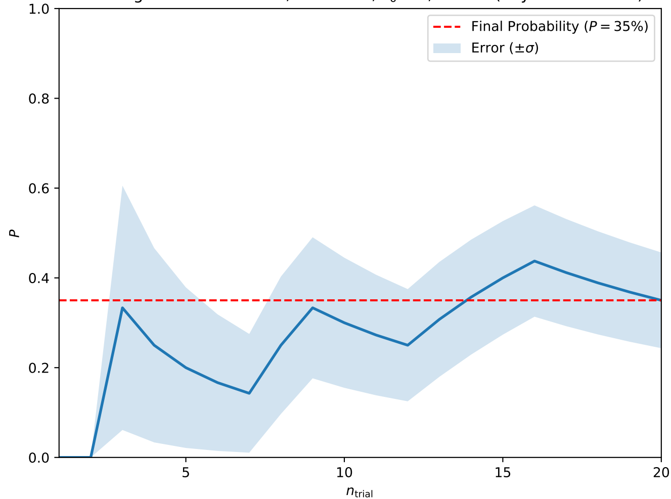
Convergence at A = 0.225, H = 0.275, T_0 = 3, w = 10 (Skyrmion Lattice)
