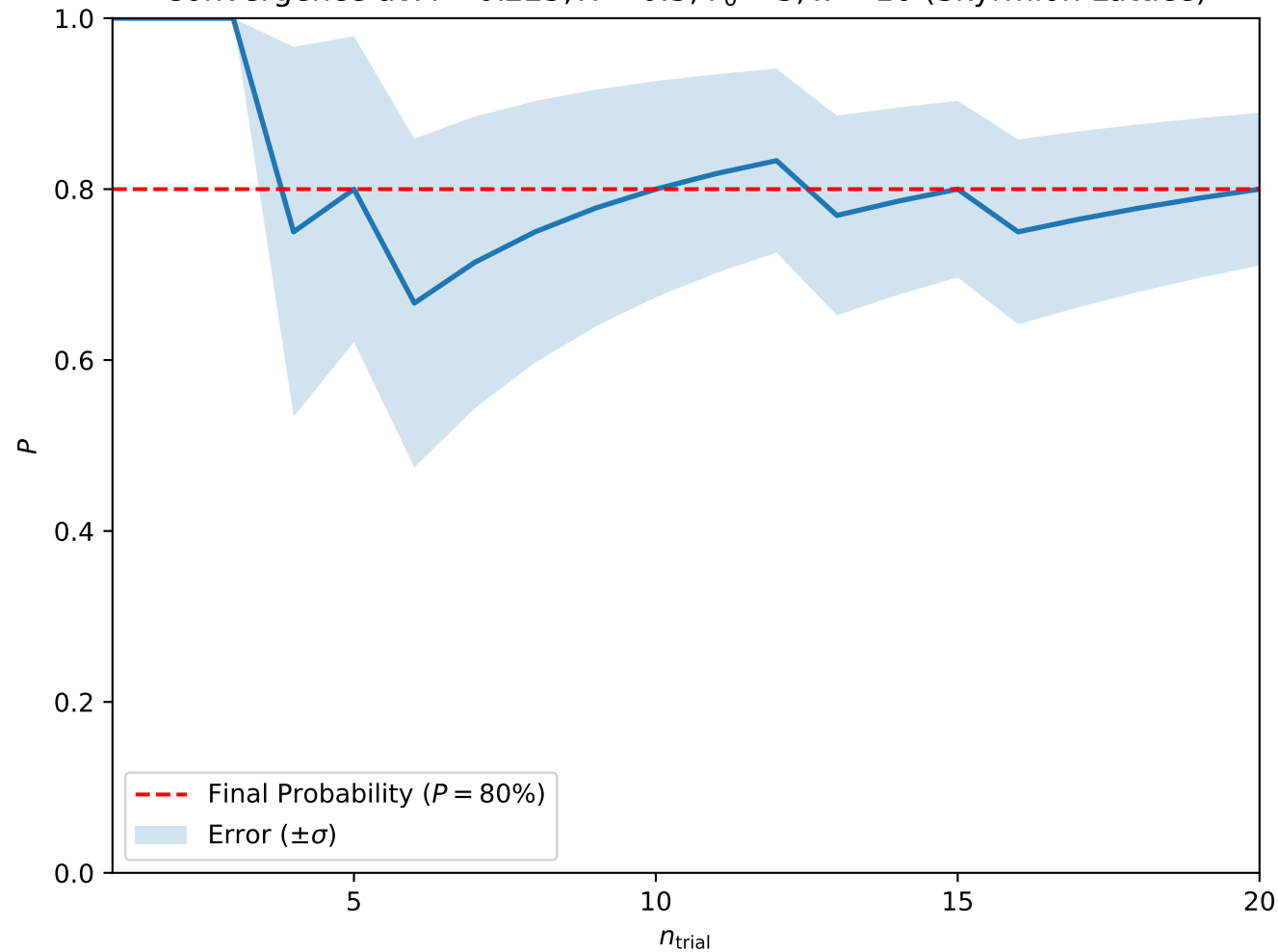
Convergence at A = 0.225, H = 0.3, T_0 = 3, w = 10 (Skyrmion Lattice)
