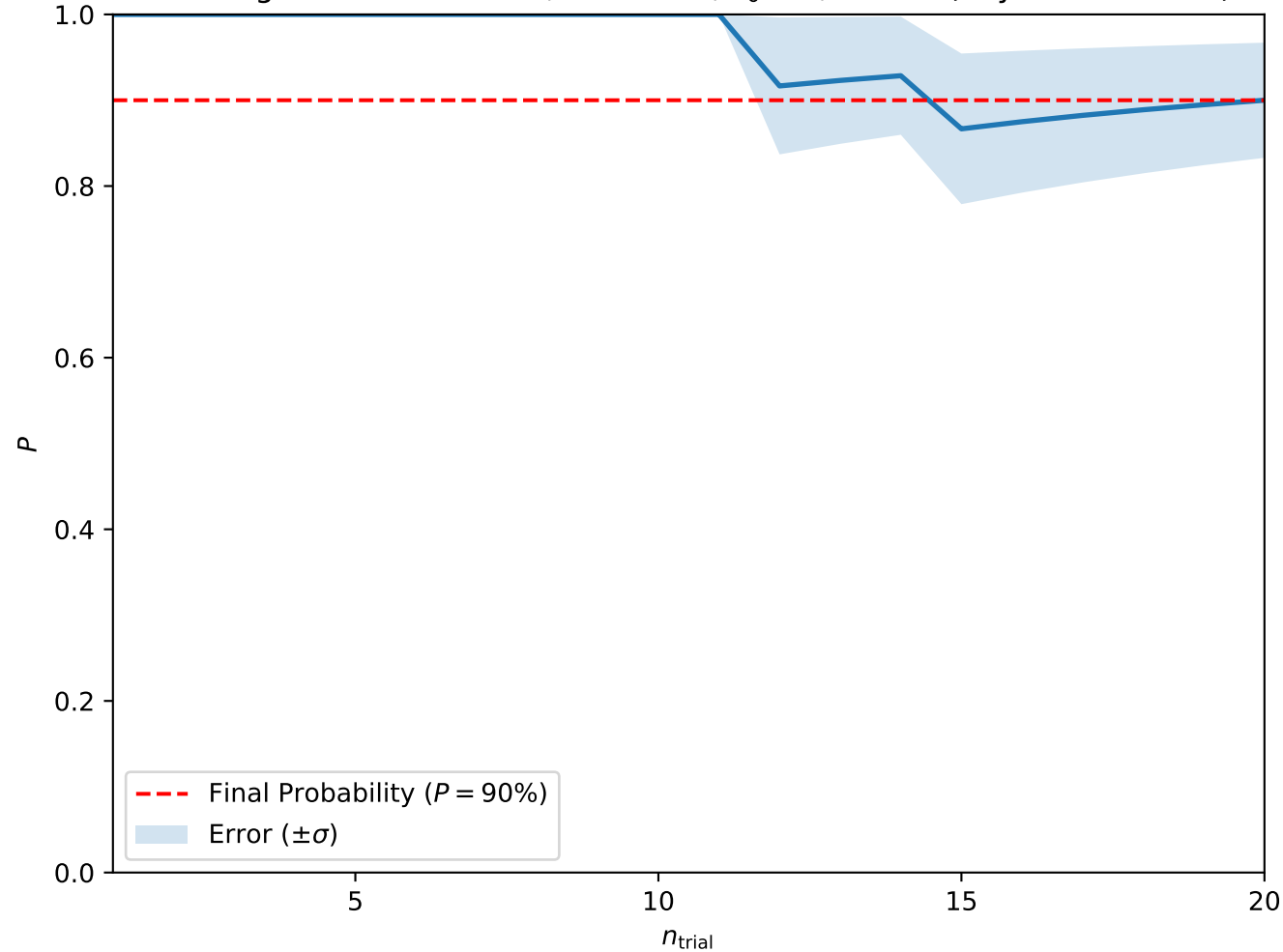
Convergence at A = 0.225, H = 0.325, T_0 = 3, w = 10 (Skyrmion Lattice)
