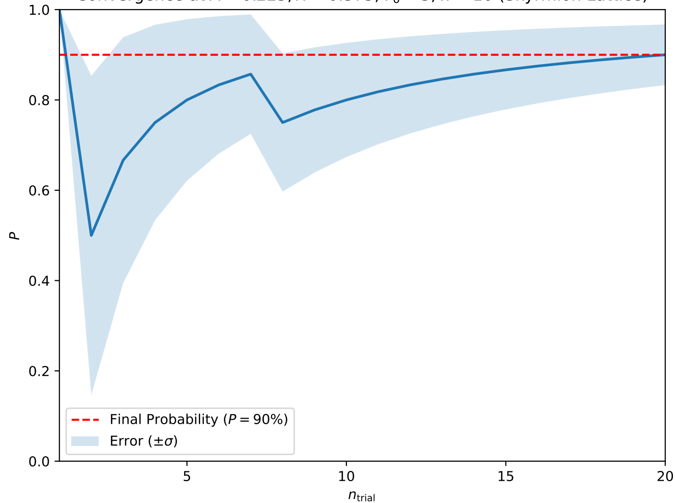
Convergence at A = 0.225, H = 0.375, T_0 = 3, w = 10 (Skyrmion Lattice)
