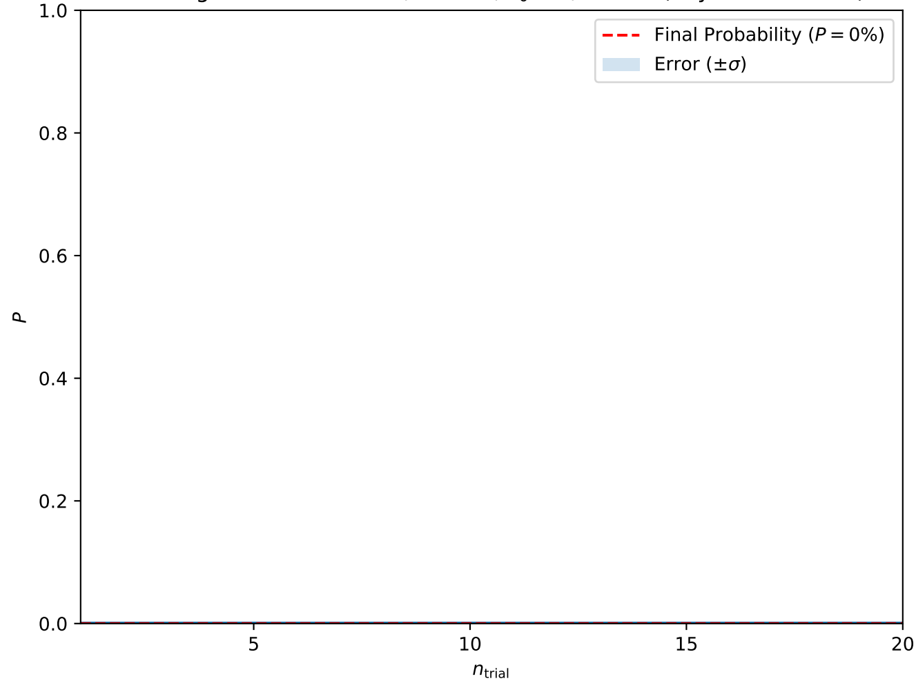
Convergence at A = 0.225, H = 0.6, T_0 = 3, w = 10 (Skyrmion Lattice)
