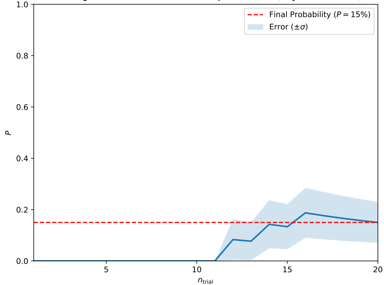
Convergence at A = 0.25, H = 0.25, T_0 = 3, w = 10 (Skyrmion Lattice)
