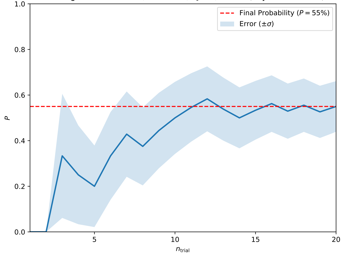
Convergence at A = 0.25, H = 0.275, T_0 = 3, w = 10 (Skyrmion Lattice)
