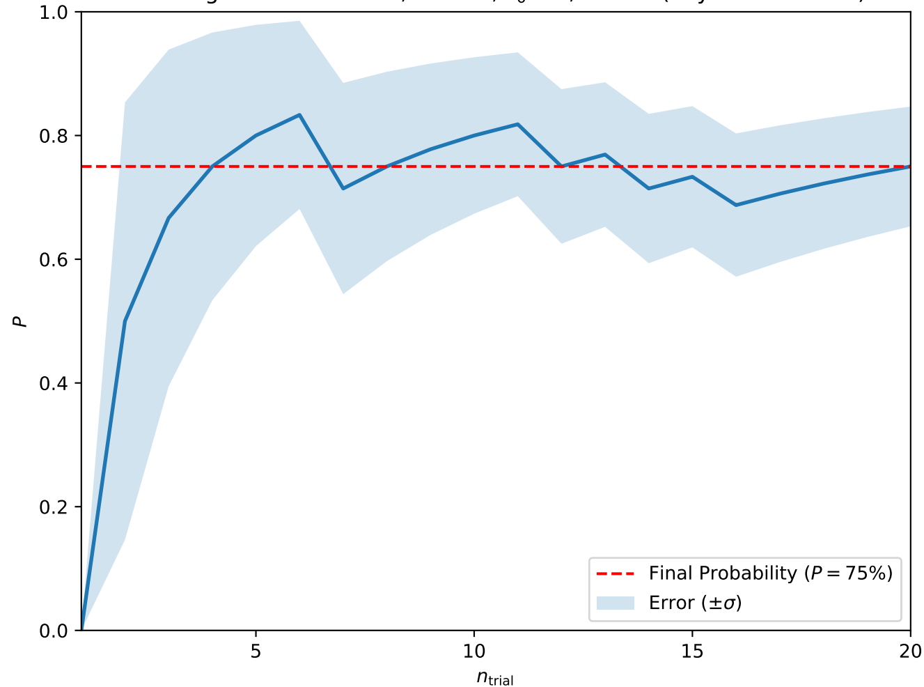
Convergence at A = 0.25, H = 0.3, T_0 = 3, w = 10 (Skyrmion Lattice)
