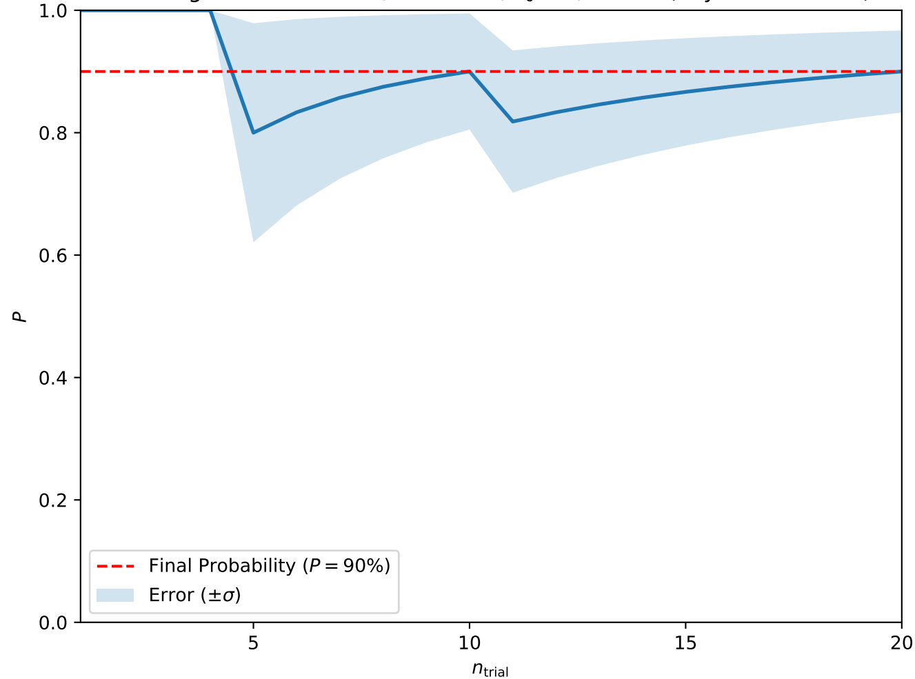
Convergence at A = 0.25, H = 0.325, T_0 = 3, w = 10 (Skyrmion Lattice)
