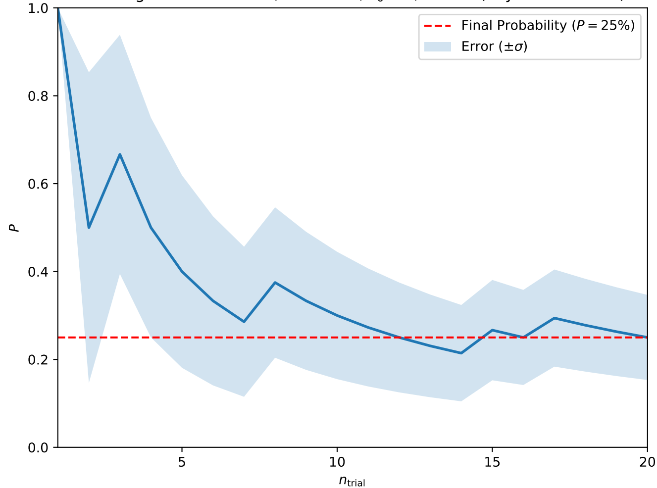
Convergence at A = 0.25, H = 0.375, T_0 = 3, w = 10 (Skyrmion Lattice)
