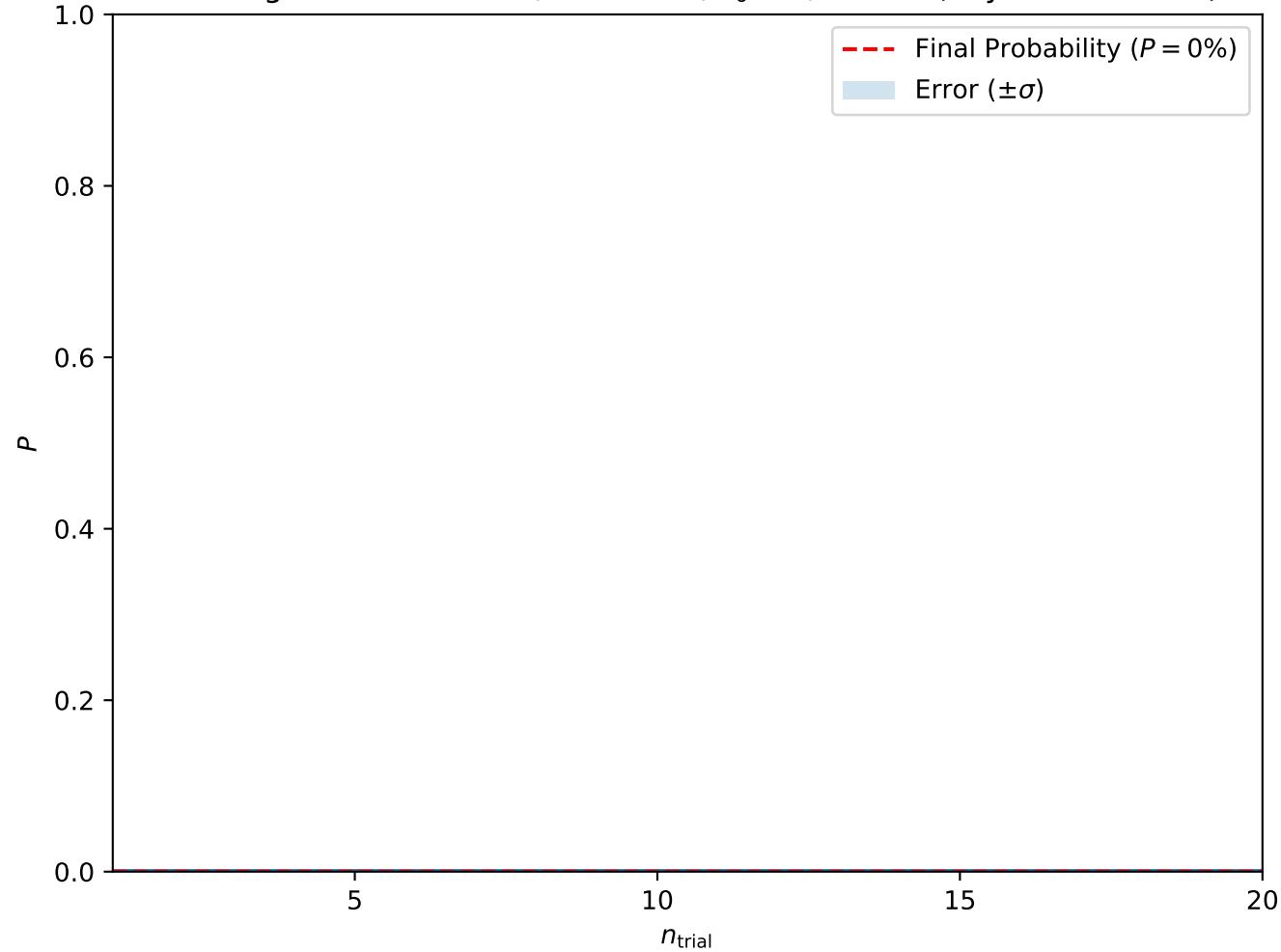
Convergence at A = 0.25, H = 0.525, T_0 = 3, w = 10 (Skyrmion Lattice)
